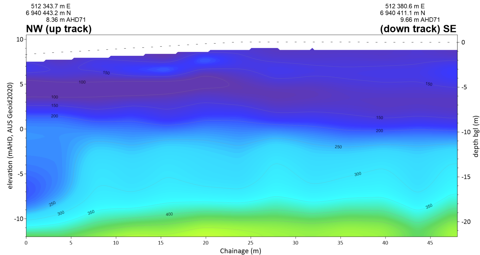
Seismic Line MASW AU-GP 145-2
